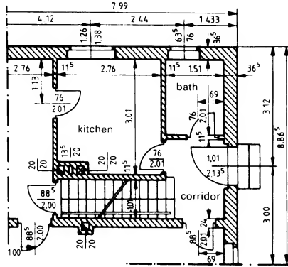
2 Construction drawing
